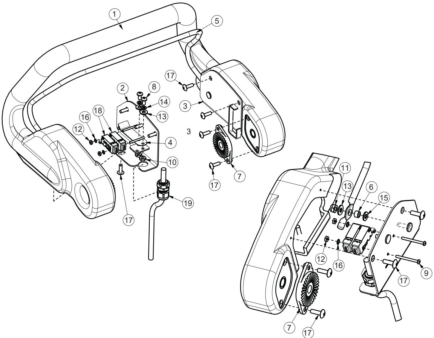
BILL OF MATERIAL - 172015
